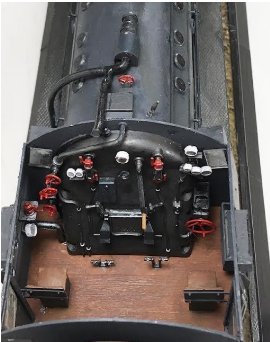
Interior photos of Arthur Berdick's German Locomotive and Tender
