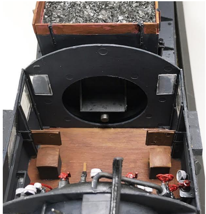
Interior photos of Arthur Berdick's German Locomotive and Tender
