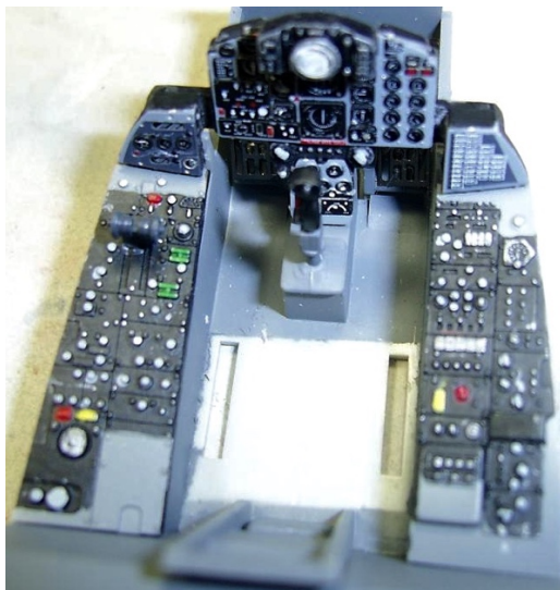
Front Cockpit of F-4J
